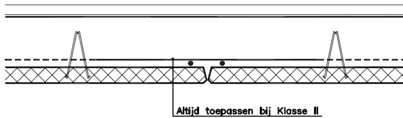
Detail IX
