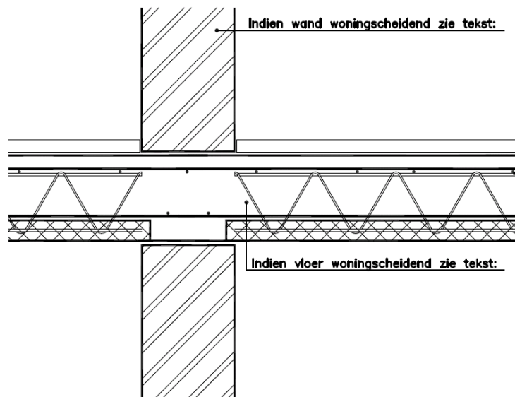
Detail 2
