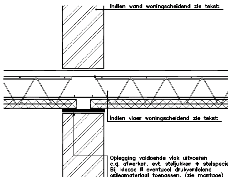
Detail 2a
